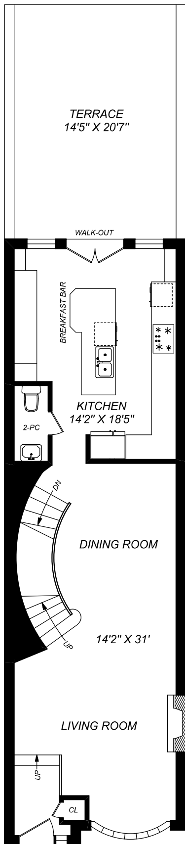
MAIN FLOOR 822 SQUARE FEET CEILING HEIGHT = 9'-0"
